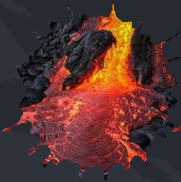
Lava Domes
